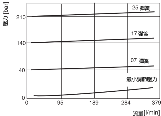
RM6 壓力曲綫
