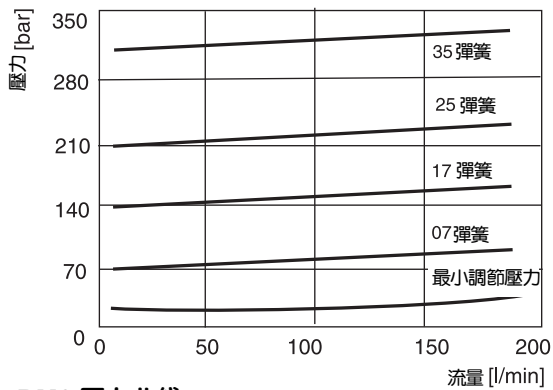
RM6 壓力曲綫
