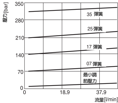
RM3 壓力曲綫
